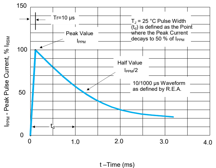
FIGURE 4 Pulse Waveform
